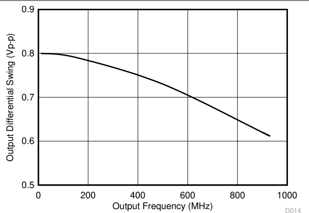
Figure 6-14. LVDS Differential Output Swing vs Frequency
