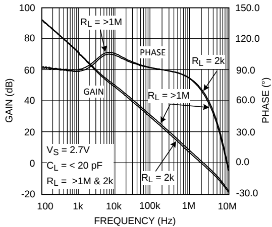
Figure 19. Open Loop Gain and Phase vs R_L at 2.7 V
