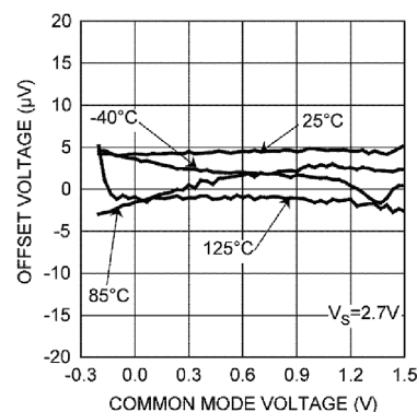
Offset Voltage vs Common Mode Voltage
