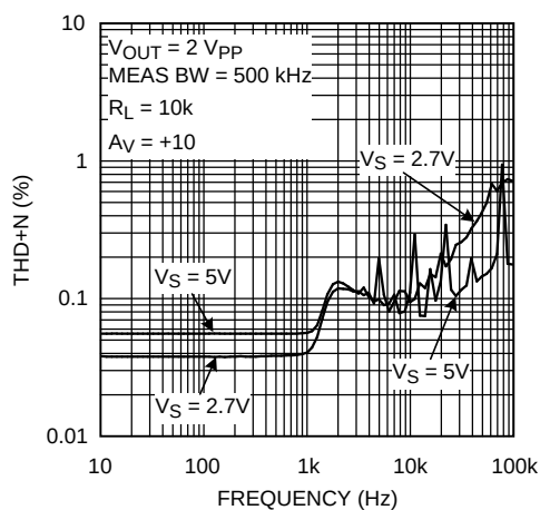
Figure 26. THD+N vs Frequency
