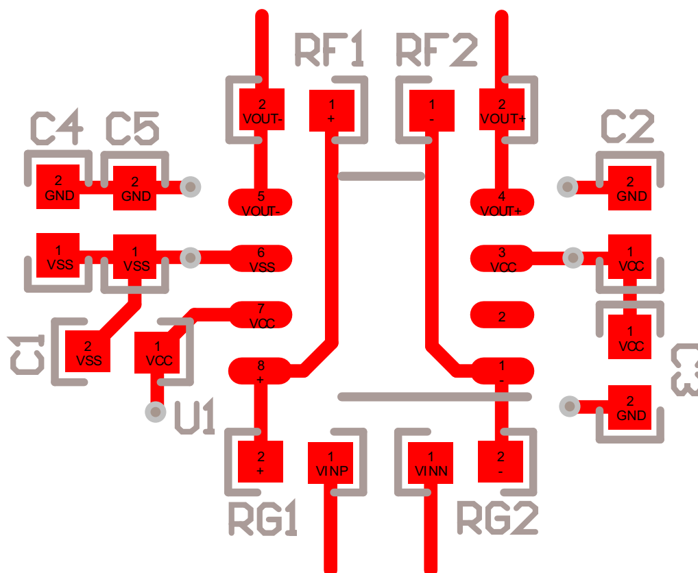
Figure 38. Layout Example
