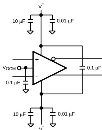
Figure 36. Split-Supply Bypassing Capacitors
