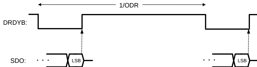
Figure 61. DRDYB Behavior for a Complete ADC_DOUT Reading
