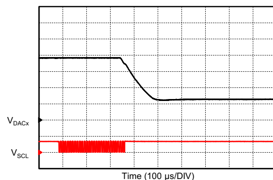
DAC OVERRIDE MODE C_L = 10\text{ pF} I^2C command triggers DAC step Step size: 3/4 to 1/4 FS
