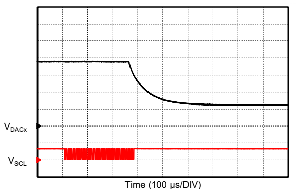
DAC OVERRIDE MODE C_L = 10\text{ }\mu\text{F} I^2C command triggers DAC step Step size: 3/4 to 1/4 FS
