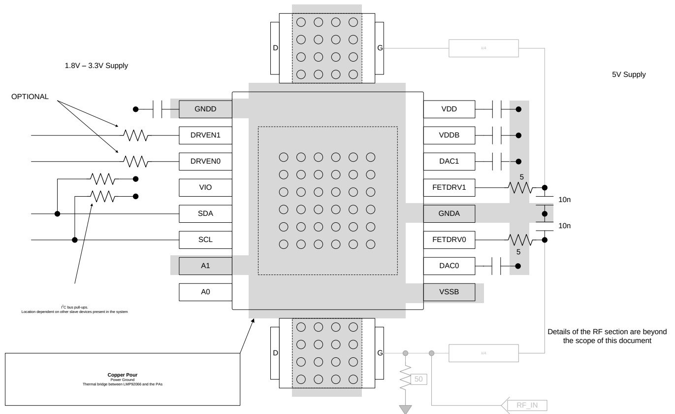
Figure 53. LMP92066 Layout
