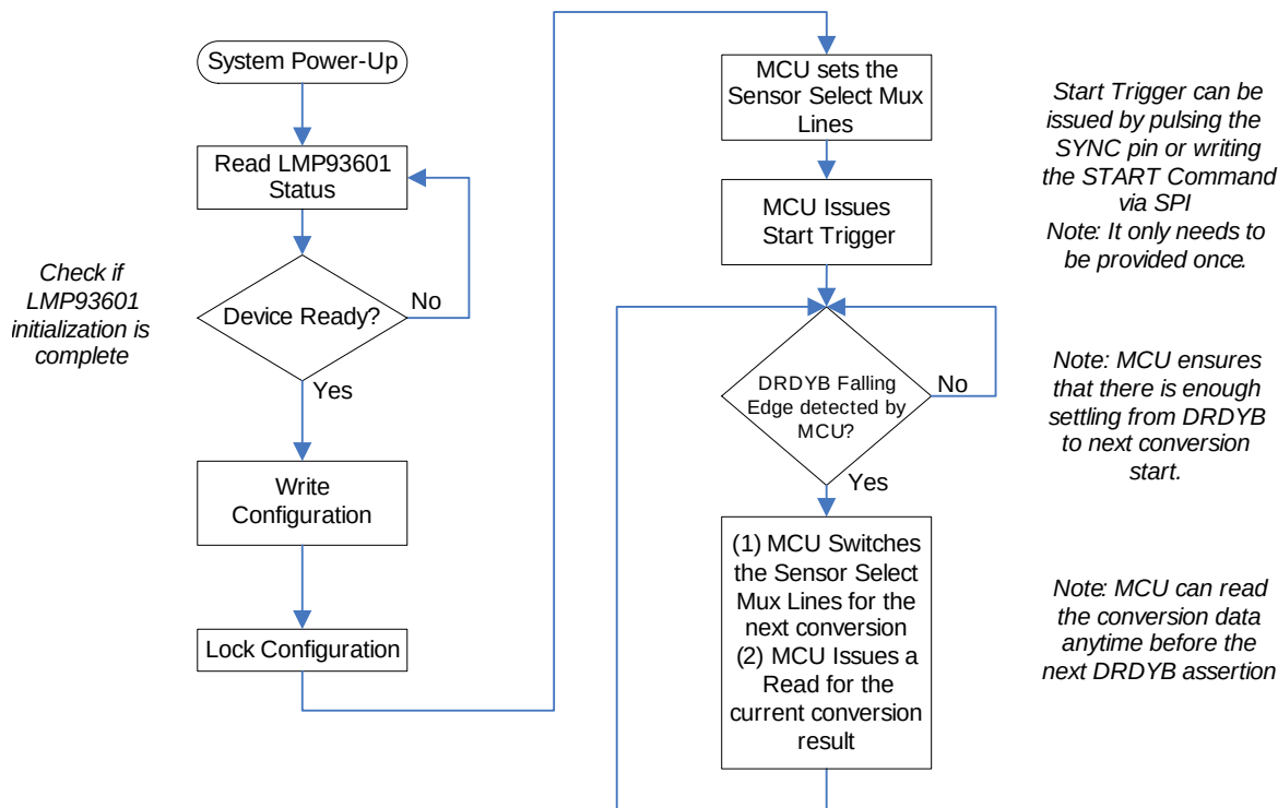
Figure 21. Continuous Mode Flow Chart
