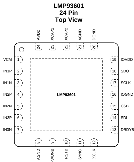
Pin Functions
