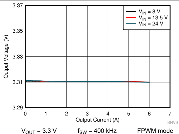
Figure 8-14. LMQ61460-Q1 Load and Line Regulation
