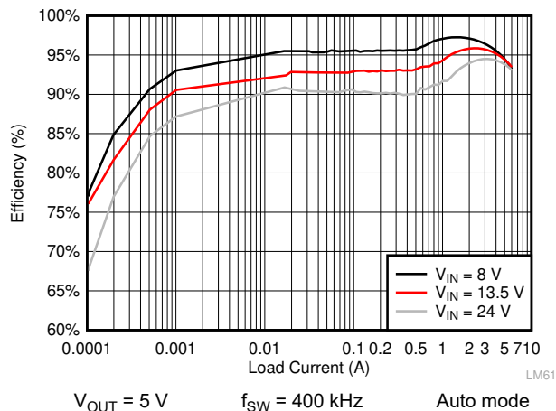
Figure 8-9. LMQ61460-Q1 Efficiency
