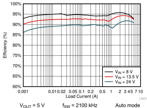
Figure 8-11. LMQ61460-Q1 Efficiency
