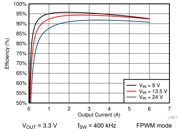
Figure 8-6. LMQ61460-Q1 Efficiency
