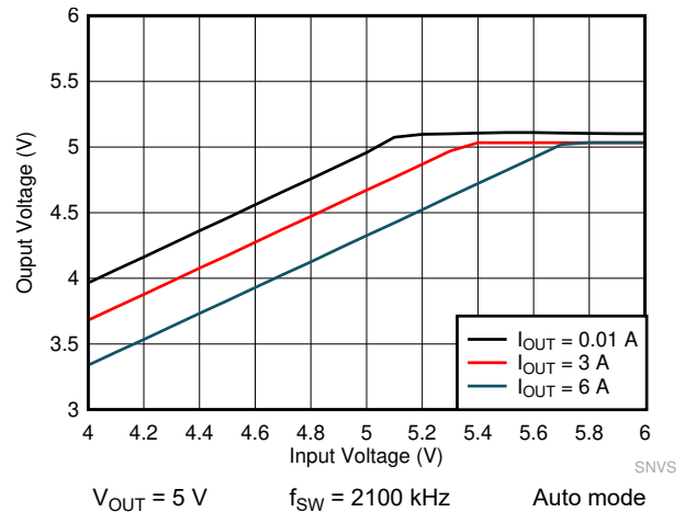
Figure 8-24. LMQ61460-Q1 Dropout Curve
