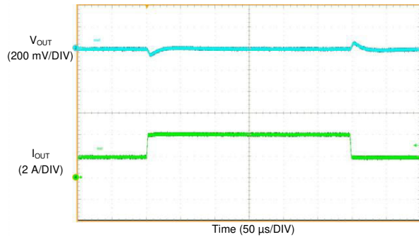
Figure 8-41. LMQ61460-Q1 Load Transient
