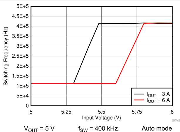
Figure 8-27. LMQ61460-Q1 Frequency Dropout Curve
