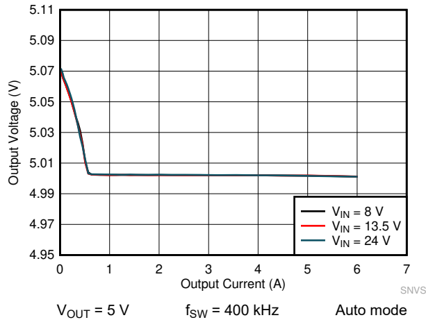
Figure 8-17. LMQ61460-Q1 Load and Line Regulation
