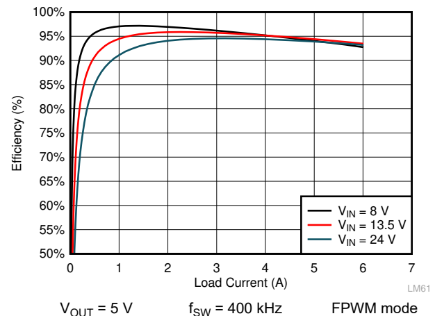
Figure 8-10. LMQ61460-Q1 Efficiency
