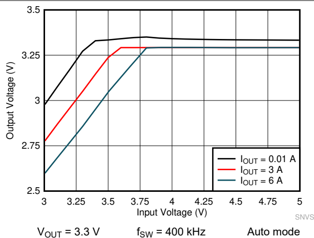
Figure 8-21. LMQ61460-Q1 Dropout Curve
