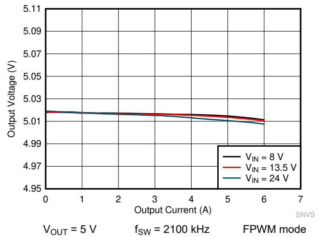
Figure 8-20. LMQ61460-Q1 Load and Line Regulation
