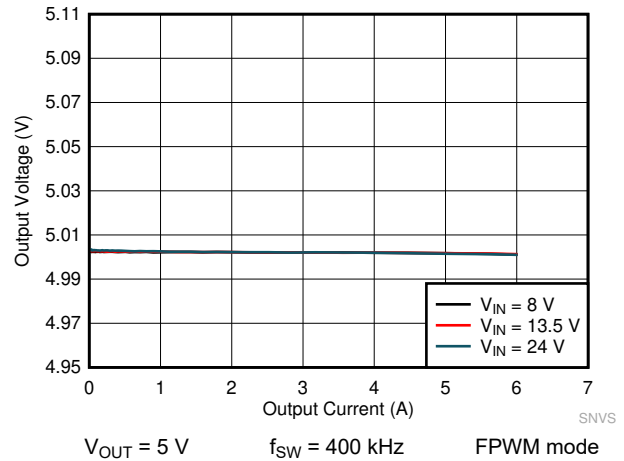
Figure 8-18. LMQ61460-Q1 Load and Line Regulation
