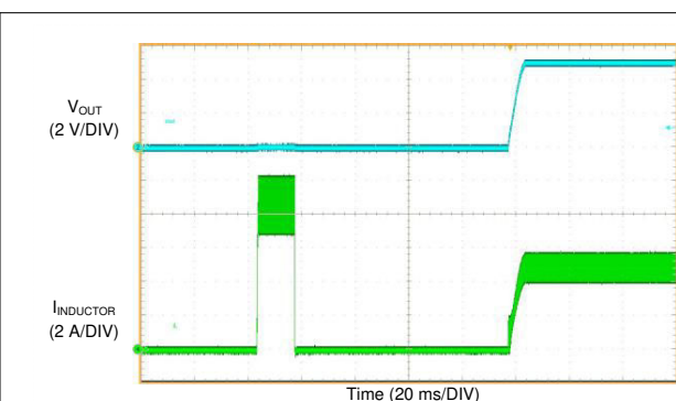
Figure 7-15. Short-Circuit Recovery
