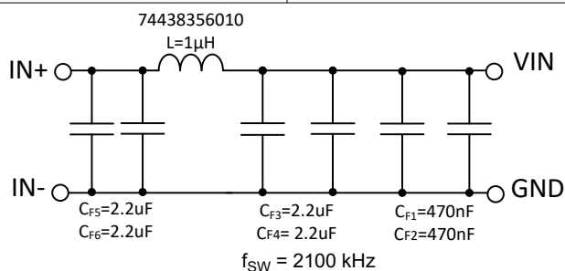
Figure 8-61. Recommended Input EMI Filter
