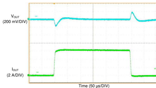
Figure 8-43. LMQ61460-Q1 Load Transient
