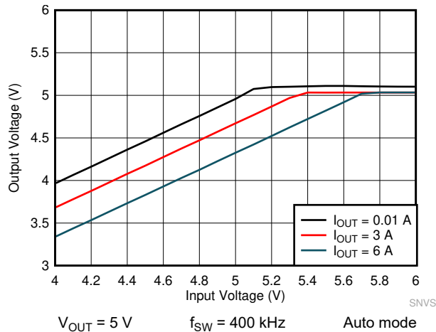
Figure 8-23. LMQ61460-Q1 Dropout Curve
