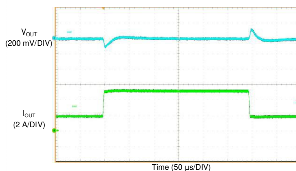
Figure 8-38. LMQ61460-Q1 Load Transient
