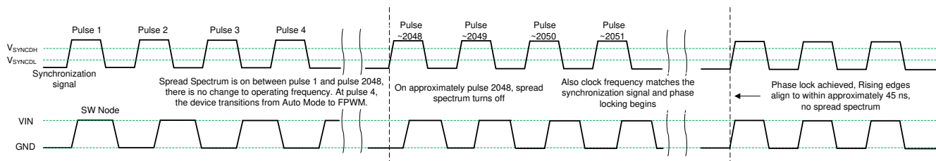
Figure 7-5. Synchronization Process
