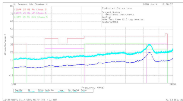
V_{OUT} = 5V f_{SW} = 2.1MHz I_{OUT} = 4A Frequency Tested: 300MHz to 1GHz
