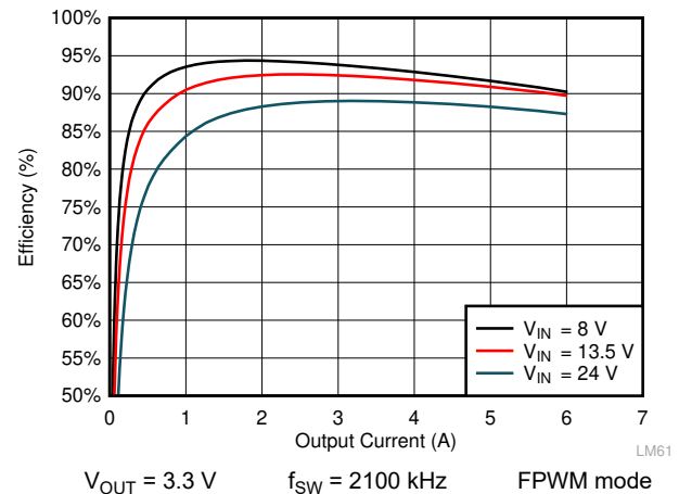
Figure 8-8. LMQ61460-Q1 Efficiency
