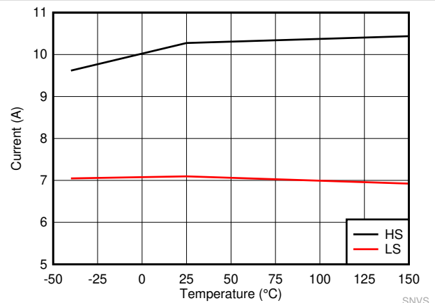
Figure 6-4. LMQ61460-Q1 High-Side and Low-Side Current Limits
