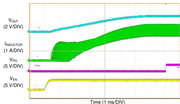
Figure 8-31. LMQ61460-Q1 Start-Up With 50mA Load
