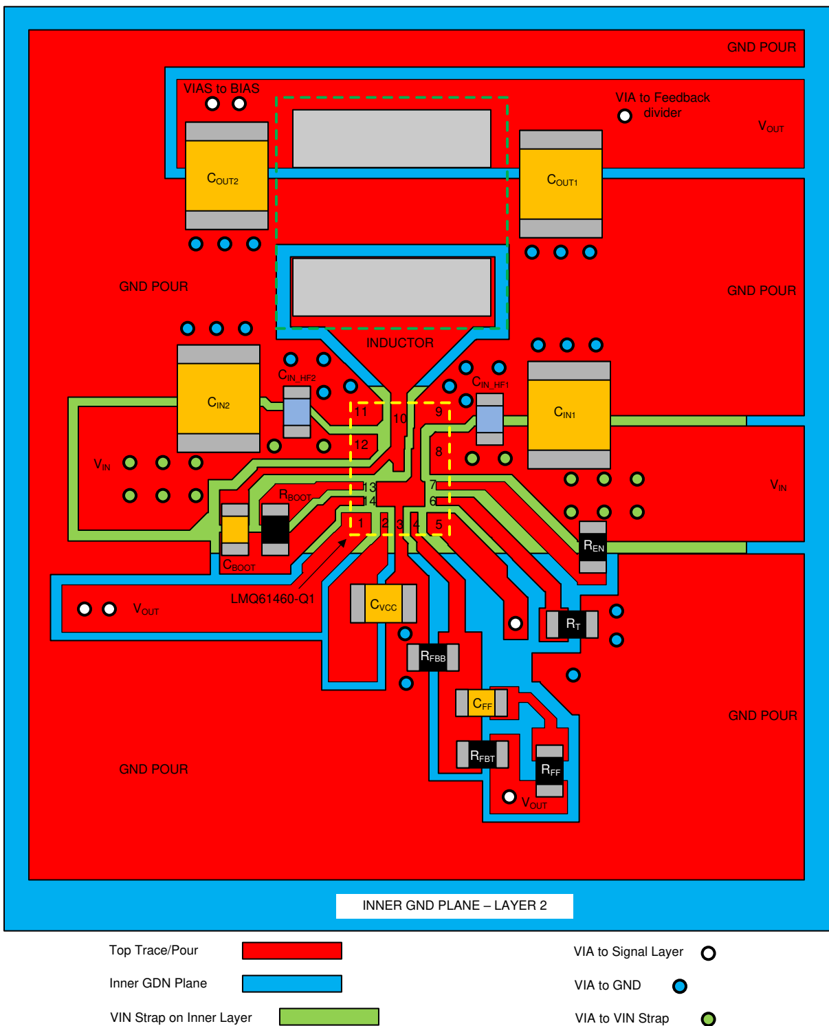
Figure 8-63. Layout Example
