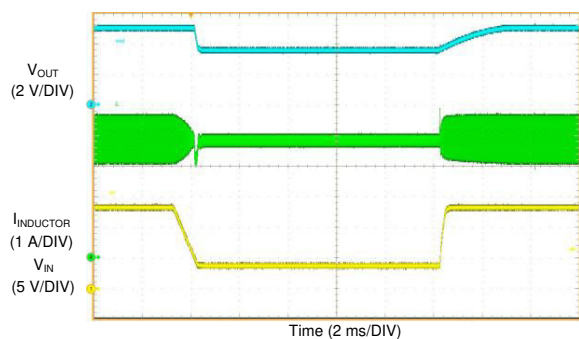
Figure 8-35. LMQ61460-Q1 Short-Circuit Recovery
