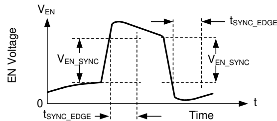
Figure 7-3. Typical SYNC/EN Waveform
