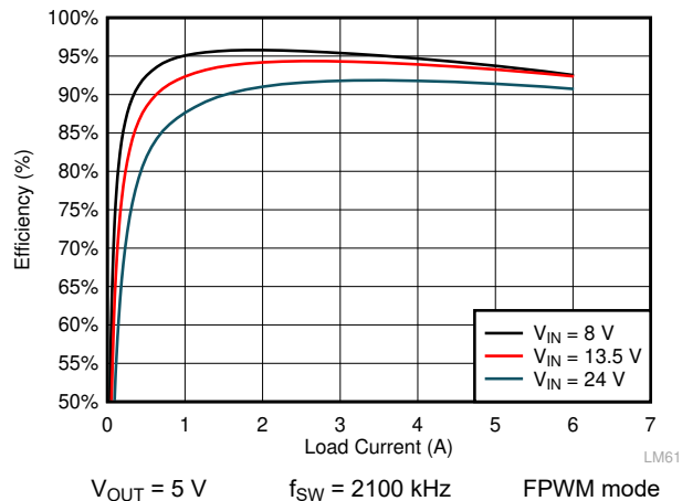
Figure 8-12. LMQ61460-Q1 Efficiency
