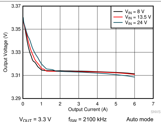
Figure 8-15. LMQ61460-Q1 Load and Line Regulation
