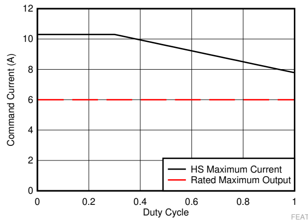
Figure 7-12. Maximum Current Allowed Through the HS FET - Function of Duty Cycle for LMQ61460-Q1
