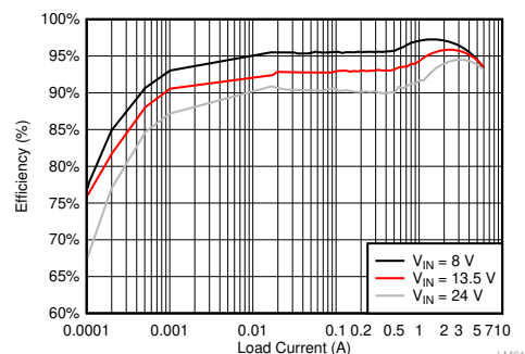
Efficiency: V_{\text{OUT}} = 5\text{V} , F_{\text{SW}} = 400\text{kHz}
