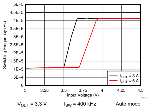
Figure 8-25. LMQ61460-Q1 Frequency Dropout Curve
