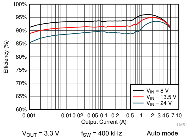
Figure 8-5. LMQ61460-Q1 Efficiency
