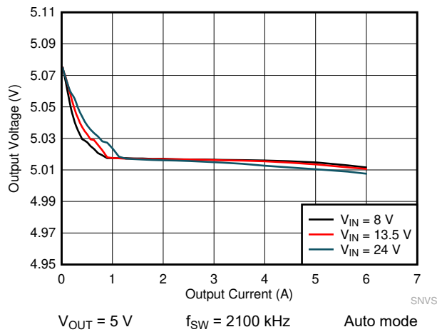
Figure 8-19. LMQ61460-Q1 Load and Line Regulation
