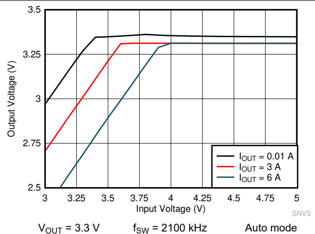
Figure 8-22. LMQ61460-Q1 Dropout Curve
