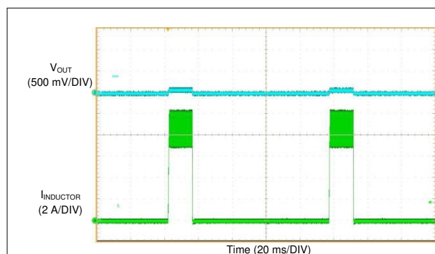
Figure 7-14. Inductor Current Bursts During Hiccup
