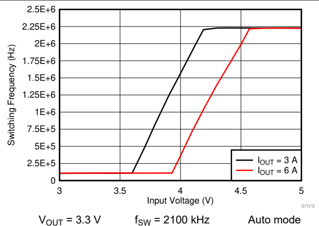
Figure 8-26. LMQ61460-Q1 Frequency Dropout Curve
