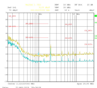
Conducted EMI: V_{\text{OUT}} = 5\text{V} , I_{\text{OUT}} = 4\text{A}
