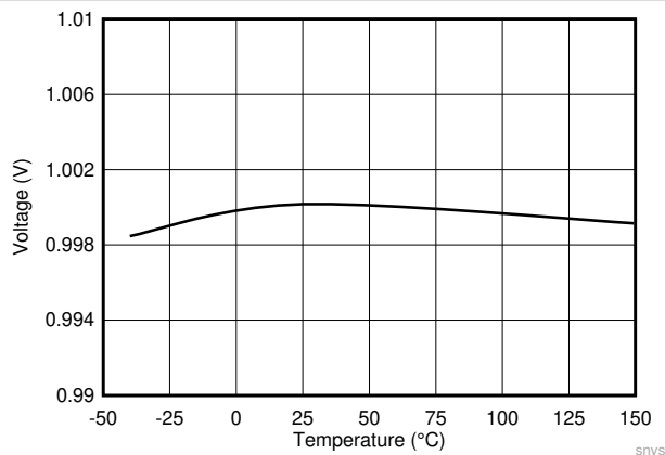
Figure 6-3. Feedback Voltage
