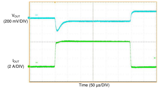
Figure 8-42. LMQ61460-Q1 Load Transient
