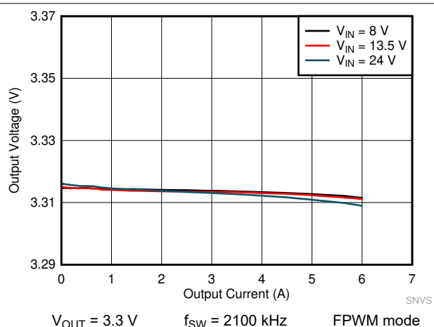
Figure 8-16. LMQ61460-Q1 Load and Line Regulation
