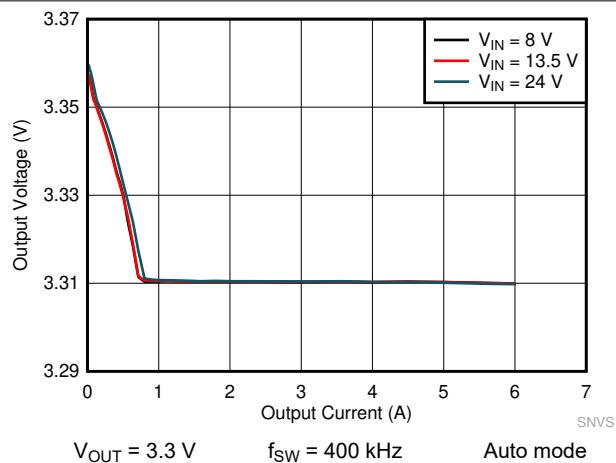
Figure 8-13. LMQ61460-Q1 Load and Line Regulation
