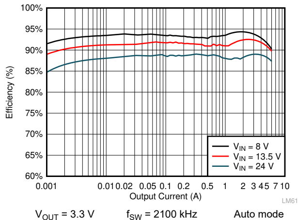
Figure 8-7. LMQ61460-Q1 Efficiency
