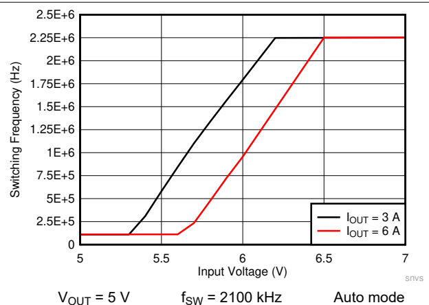
Figure 8-28. LMQ61460-Q1 Frequency Dropout Curve
