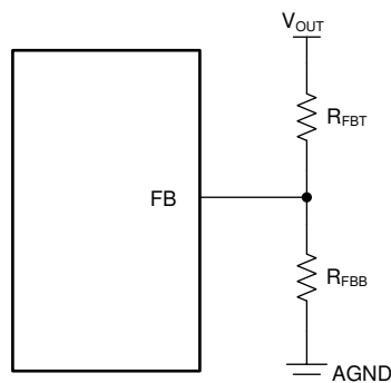
Figure 7-11. Setting Output Voltage of Adjustable Versions
