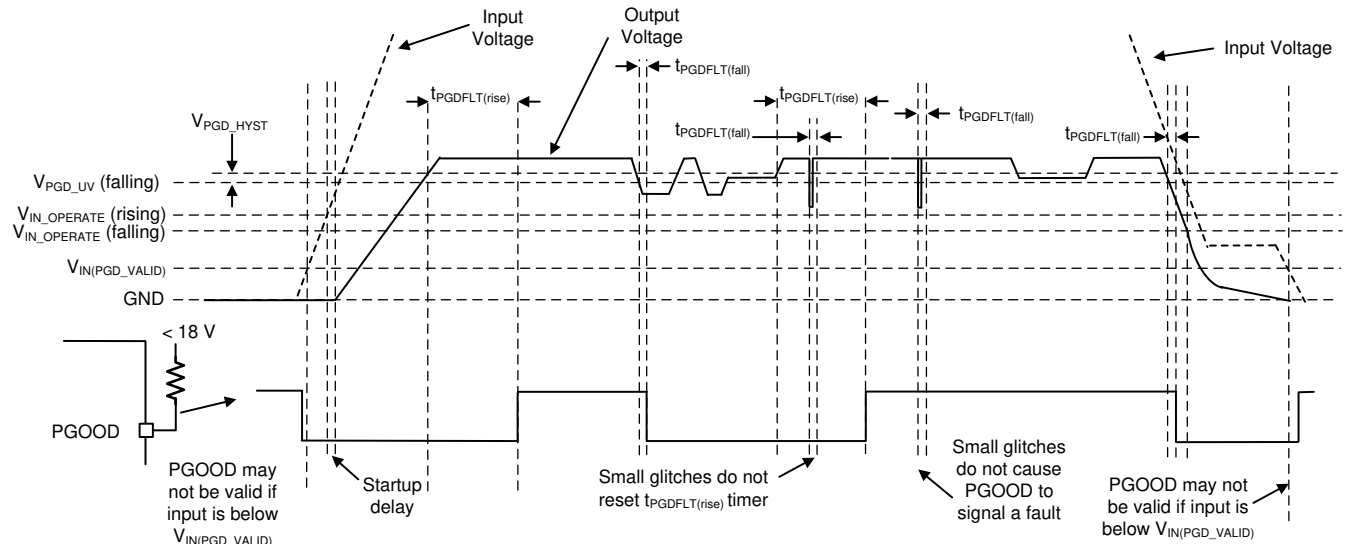
Figure 7-6. PGOOD Timing Diagram (Excludes OV Events)
