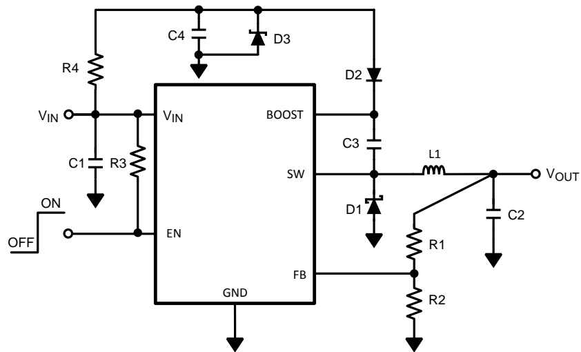
Figure 31. LMR12007Y (550kHz) V_{\text{BOOST}} Derived from V_{\text{SHUNT}} 18V to 1.5V/750mA
