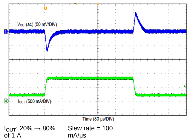
Figure 28. Load Transient
