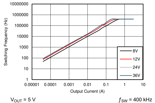
Figure 9-22. Switching Frequency versus Output Current
