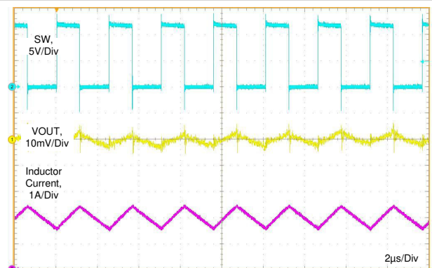
Figure 8-8. Typical PWM Switching Waveforms V_{IN} = 12\text{ V} , V_{OUT} = 5\text{ V} , I_{OUT} = 2\text{ A} , f_S = 400\text{ kHz}
