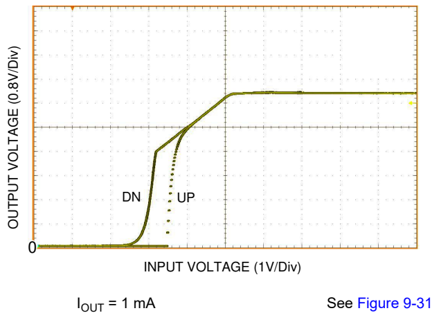
Figure 7-5. UVLO Thresholds
