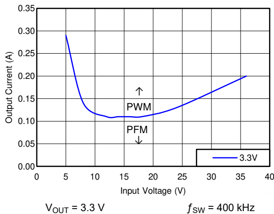
Figure 8-25. Mode Change Thresholds
