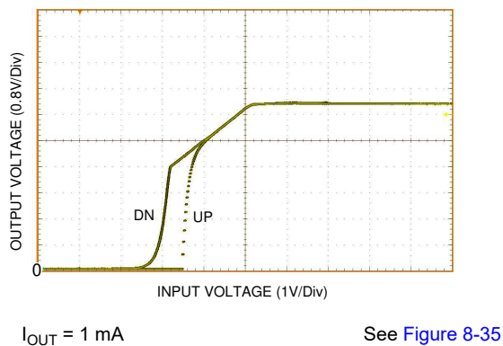
Figure 6-5. UVLO Thresholds
