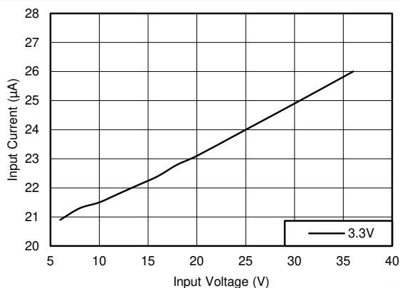
Figure 8-4. No-load Input Supply Current for 3.3-V Fixed Output Option
