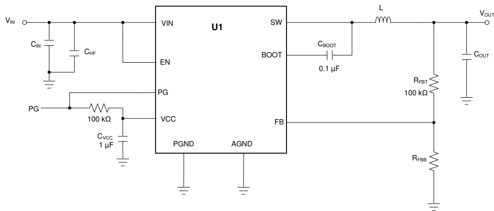
Figure 8-35. Circuit for Application Curves
