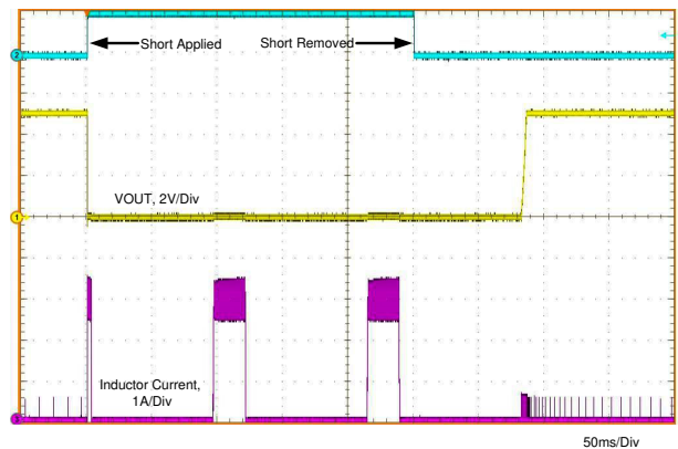
Figure 7-6. Short-Circuit Transient and Recovery
