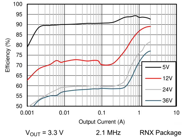
Figure 8-16. Efficiency
