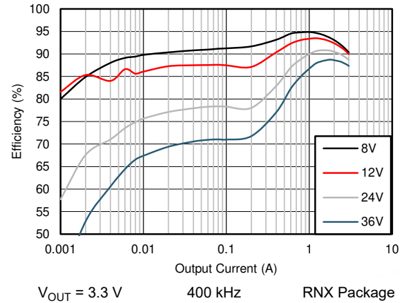
Figure 8-10. Efficiency
