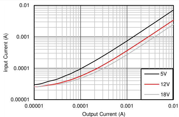
Figure 8-5. Input Supply Current vs Output Current for 3.3-V Fixed Output Option
