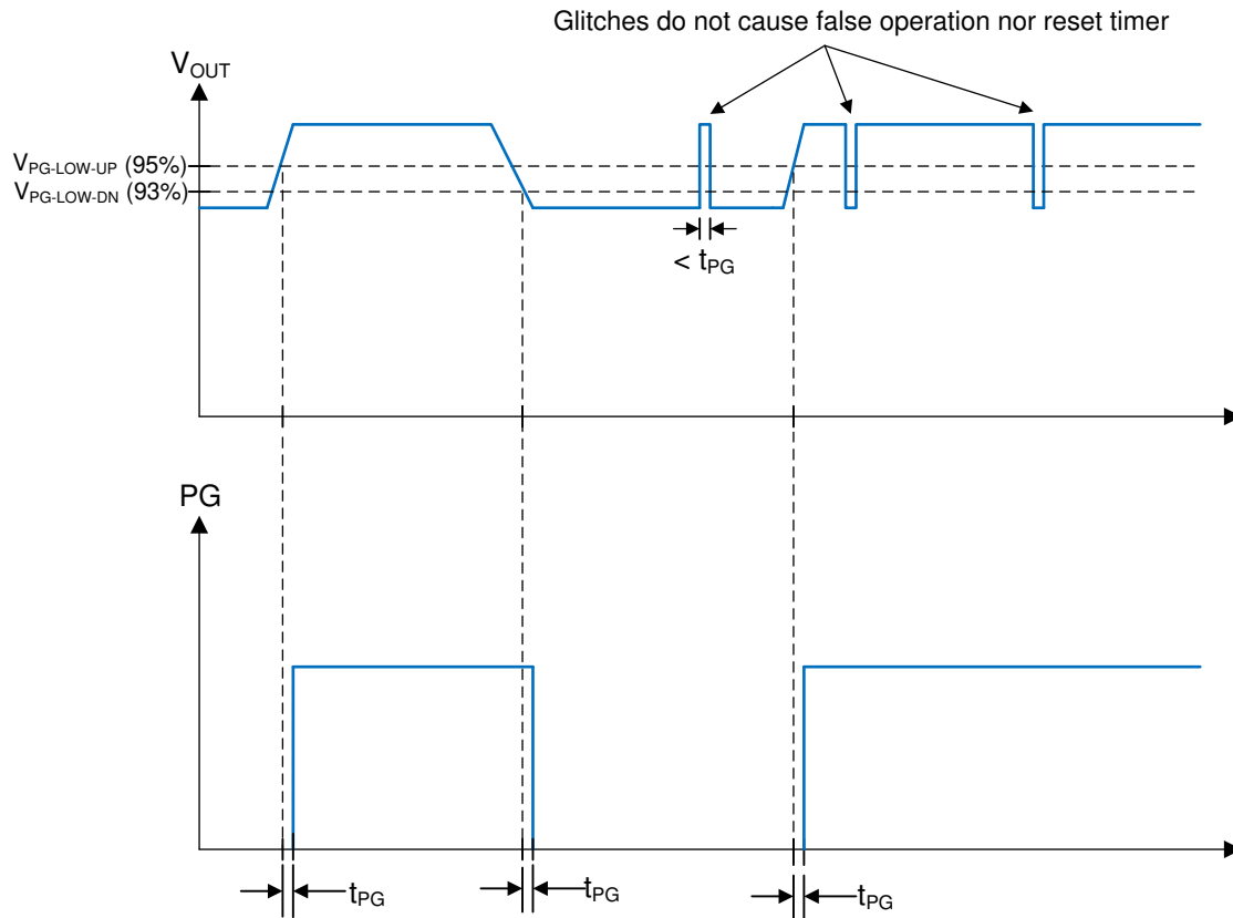
Figure 7-2. Power-Good-Timing Behavior
