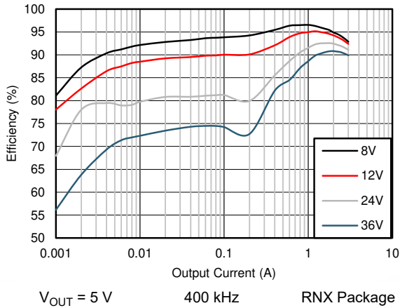
Figure 8-9. Efficiency
