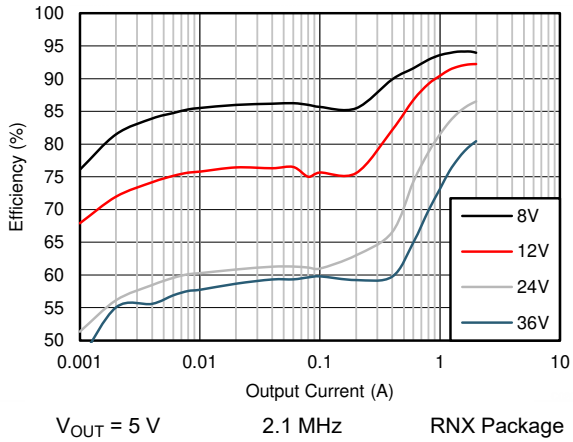
Figure 8-15. Efficiency
