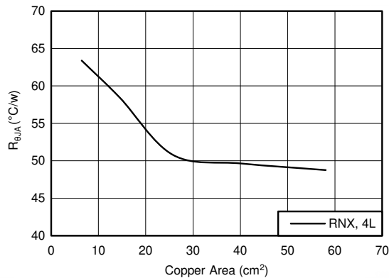
Figure 8-7. R_{\theta JA} versus Copper Board Area for the VQFN (RNX) Package
