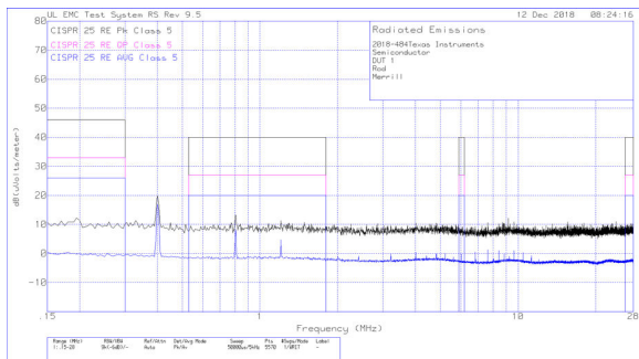
Figure 8-34. Radiated EMI Rod Antenna
