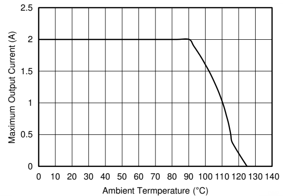
Figure 8-8. Maximum Output Current versus Ambient Temperature V_{IN} = 12\text{ V} V_{OUT} = 5\text{ V} f_{SW} = 400\text{ kHz} R_{\theta JA} = 50^{\circ}\text{C}/\text{W}
