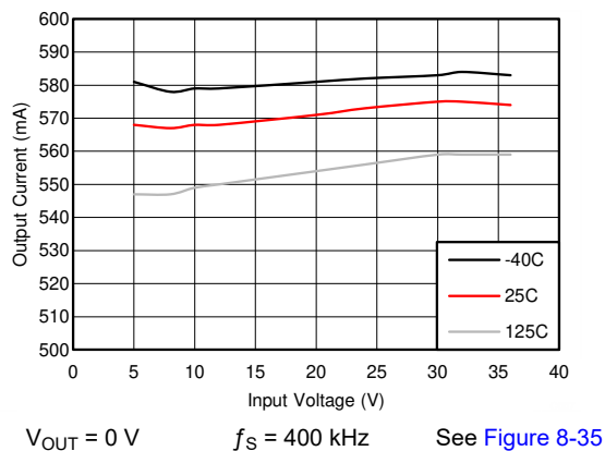
Figure 6-3. Short-Circuit Output Current
