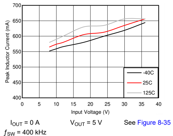
Figure 6-6. I_{PEAK-MIN}
