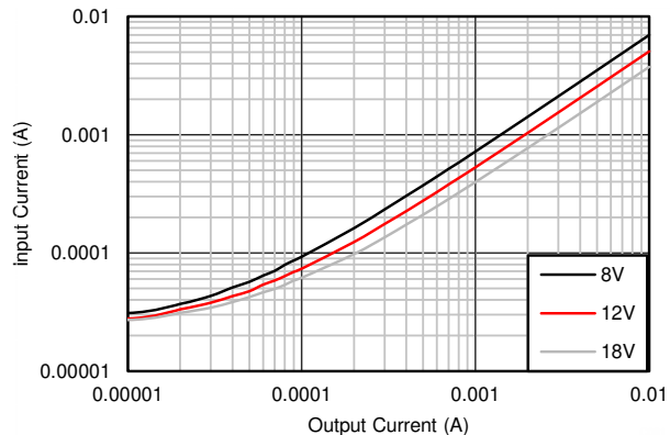
Figure 8-3. Input Supply Current vs Output Current for 5-V Fixed Output Option
