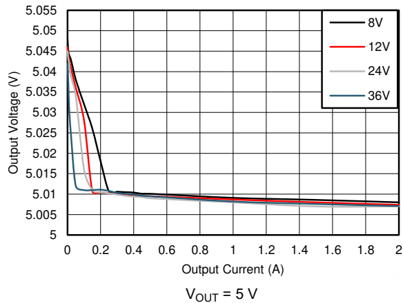
Figure 8-17. Line and Load Regulation
