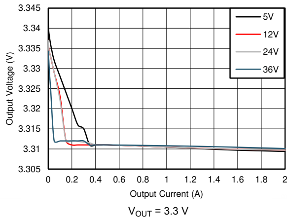
Figure 8-23. Line and Load Regulation
