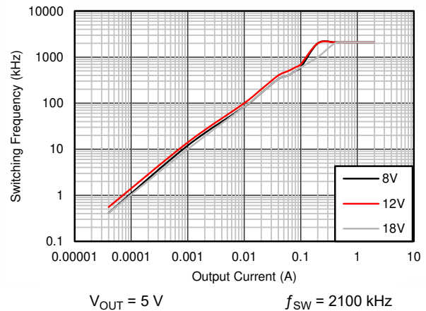
Figure 8-20. Switching Frequency versus Output Current
