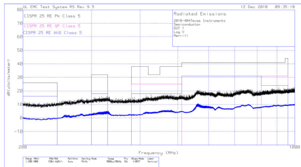
Figure 8-33. Radiated EMI Log-periodic Antenna (Vertical)
