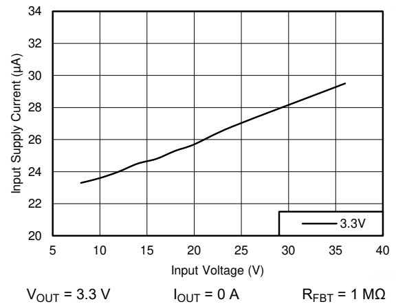
Figure 8-24. Input Supply Current
