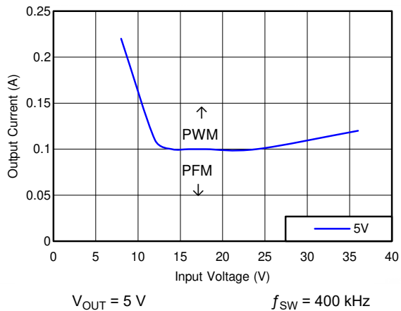
Figure 8-19. Mode Change Thresholds
