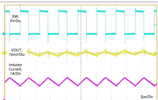
Figure 7-8. Typical PWM Switching Waveforms V_{IN} = 12\text{ V} , V_{OUT} = 5\text{ V} , I_{OUT} = 2\text{ A} , f_S = 400\text{ kHz}
