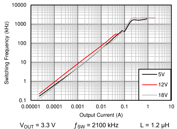
Figure 8-26. Switching Frequency versus Output Current
