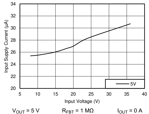
Figure 8-18. Input Supply Current
