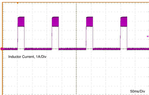
Figure 7-5. Inductor Current Burst in Short-Circuit Mode
