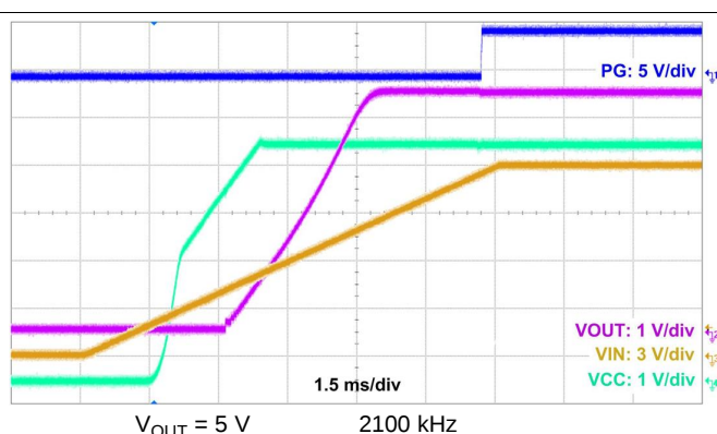
Figure 51. Start-Up Waveform
