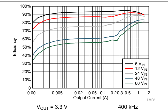
Figure 10-5. Efficiency
