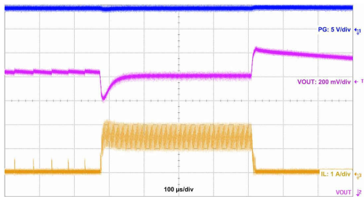
V_{OUT} = 5\text{ V} I_{LOAD} = 10\text{ mA} - 0.75\text{ A} 400 kHz Slew Rate = 1 \mu\text{s/A}
