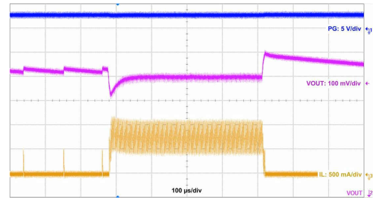
V_{OUT} = 3.3\text{ V} I_{LOAD} = 10\text{ mA} - 0.75\text{ A} 400 kHz Slew Rate = 1 \mu\text{s/A}
