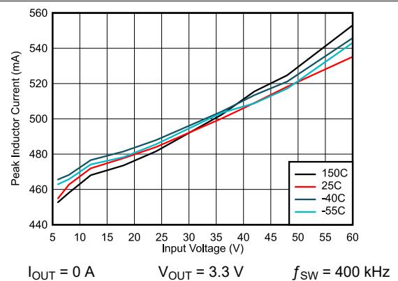
Figure 8-6. I_{PEAK-MIN}
