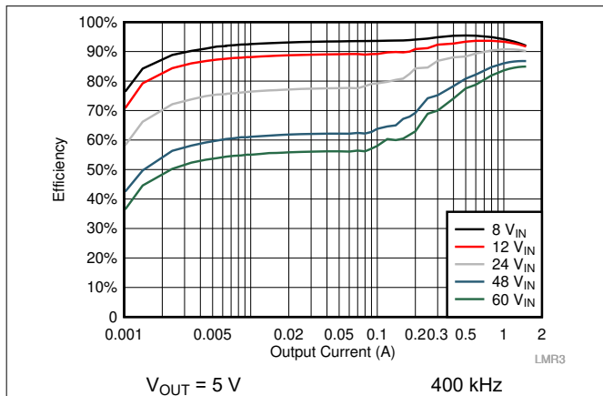
Figure 10-4. Efficiency
