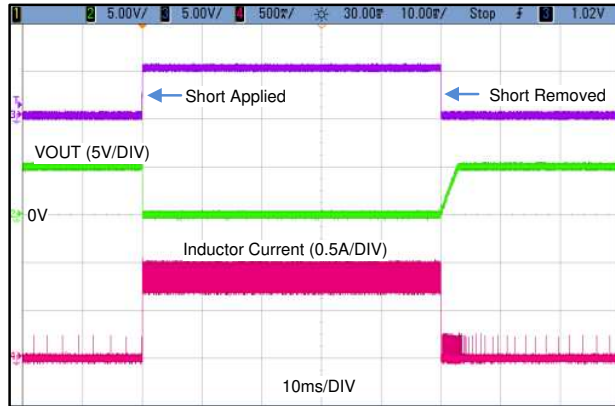
Figure 21. Short Circuit Waveform
