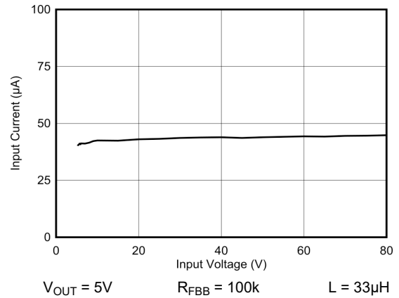
Figure 6-2. No Load Input Current vs Input Voltage
