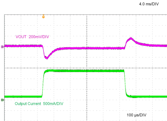
LMR38015-Q1 V_{OUT} = 5V 400kHz (AC Coupled) 150mA to 1350mA at 200mA/μs
