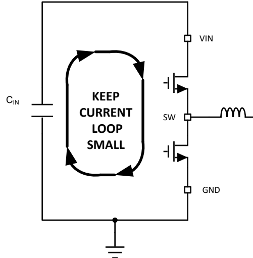
Figure 8-17. Current Loops With Fast Edges
