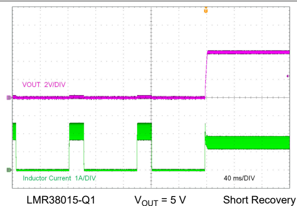
Figure 8-8. Short-Circuit Recovery
