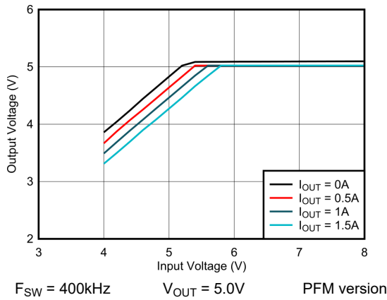
Figure 6-3. 5V Dropout
