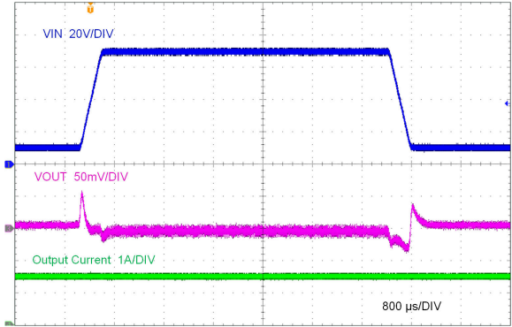
LMR38015-Q1 V_{OUT} = 5V 400kHz (AC Coupled) 10V to 70V at 200V/ms
