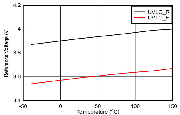
Figure 6-6. V_{IN} UVLO vs Temperature
