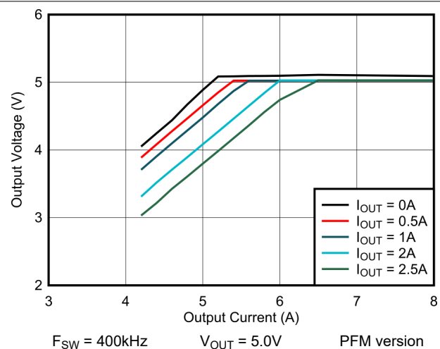
Figure 6-3. 5V Dropout
