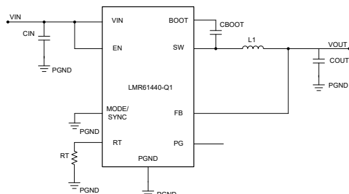
Simplified Schematic – Fixed Output
