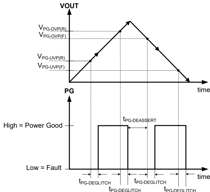
Figure 7-5. Power-Good Thresholds
