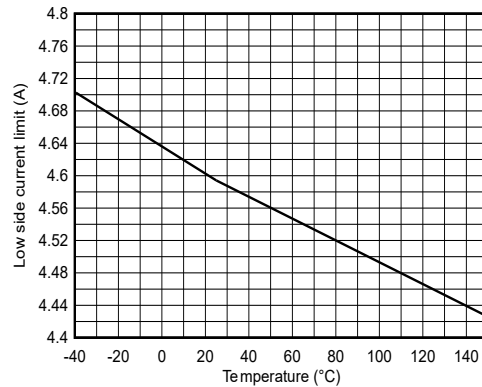
Figure 6-2. Low Side MOSFET Current Limit
