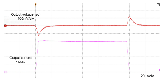
LMR61440-Q1 3.3V fixed output Mode = FPWM F_{SW} = 2MHz C_{OUT} = 1 \times 22\mu F
