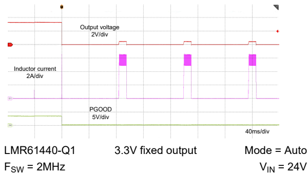
Figure 8-10. Short-Circuit Applied
