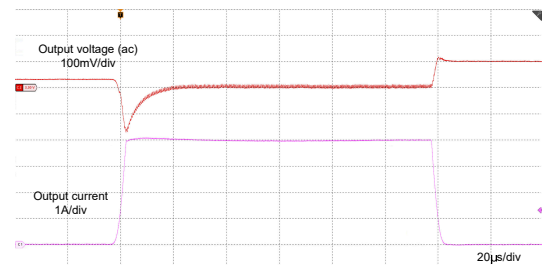
LMR61440-Q1 3.3V fixed output Mode = Auto F_{SW} = 2MHz C_{OUT} = 1 \times 22\mu F
