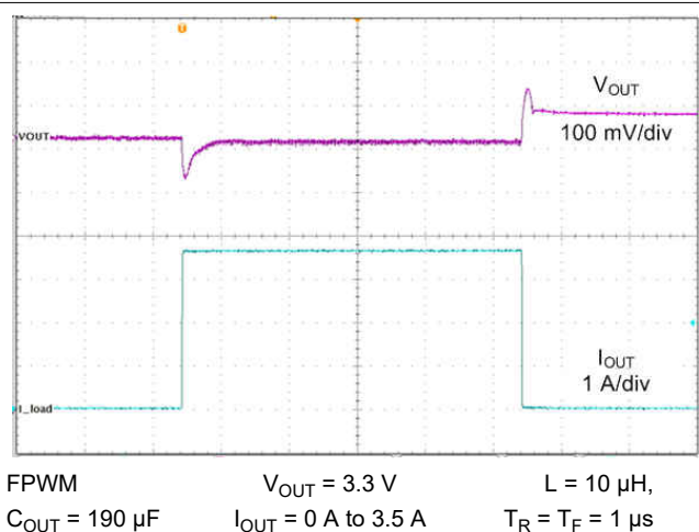
Figure 9-28. Load Transient
