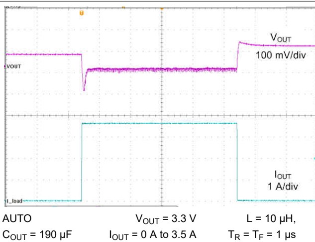
Figure 9-27. Load Transient
