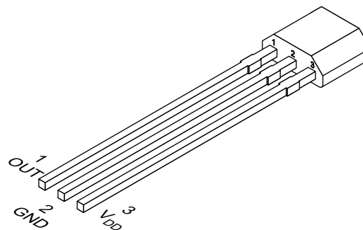
Figure 5-2. LPG Package 3-Pin TO-92S (Top View)
