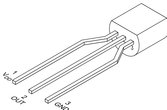
Figure 5-4. LPM Package 3-Pin TO-92 (Top View)
