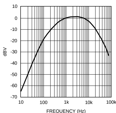
Figure 22. A-Weighted Filter
