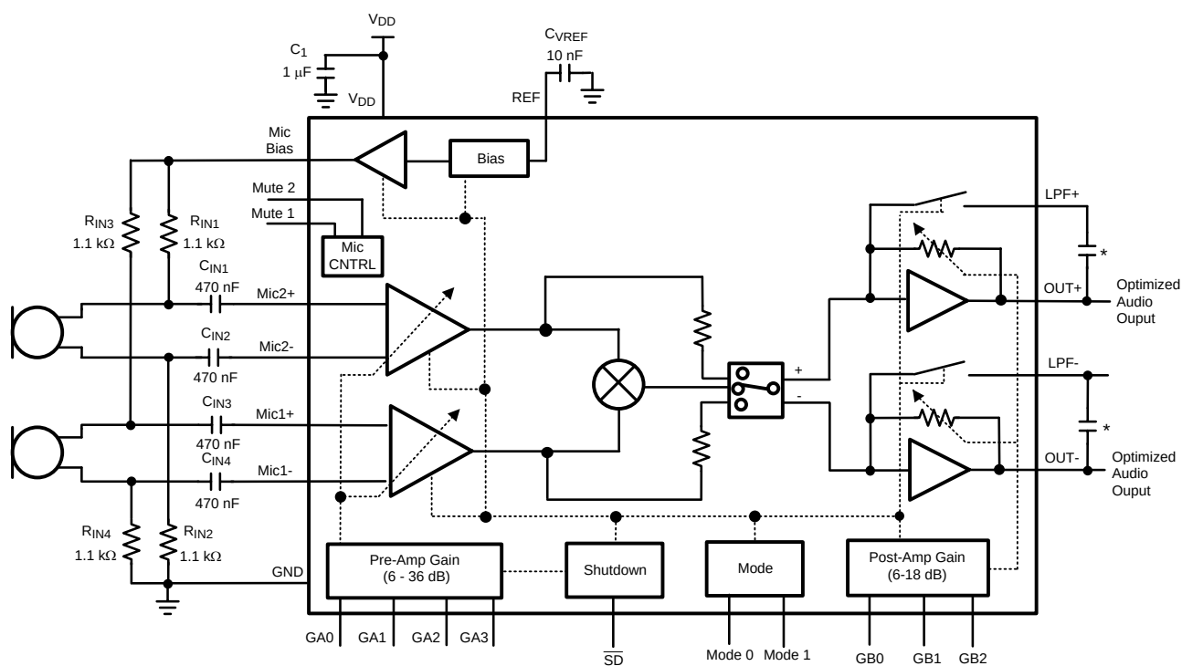
Figure 1. Typical Dual Microphone Far Field noise Cancelling Application
