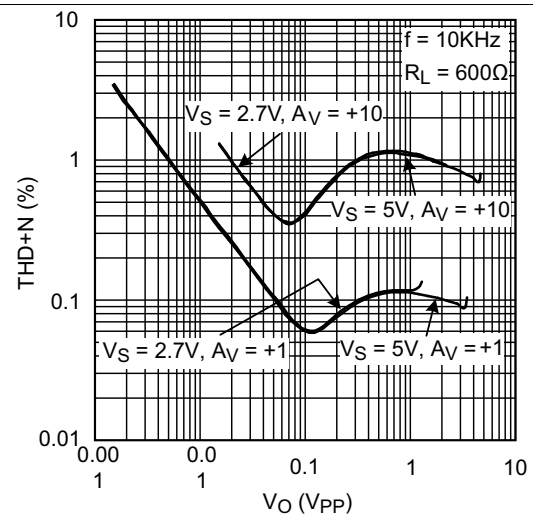
Figure 20. THD+N vs V_{O}
