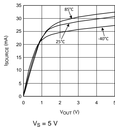
Figure 8. Sourcing Current vs Output Voltage
