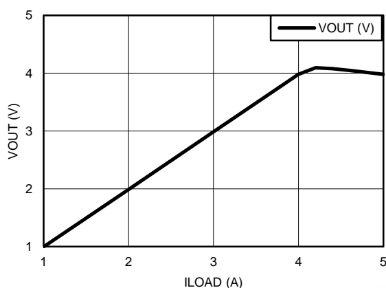
Figure 35. High-Side Current-Sensing Results
