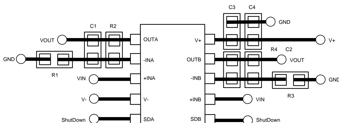
Figure 38. Sample Layout of VSSOP
