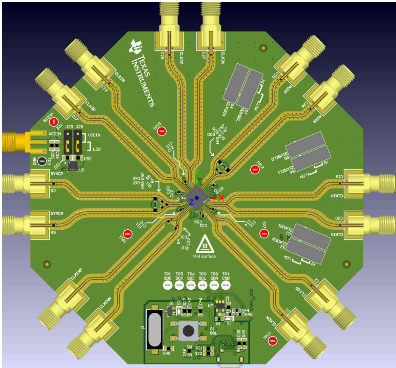
Figure 8-9. Layout Example
