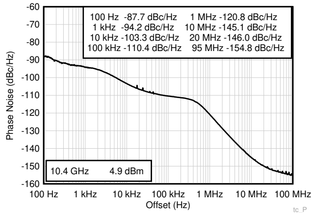
Figure 8-5. Results for Loop Filter Design
