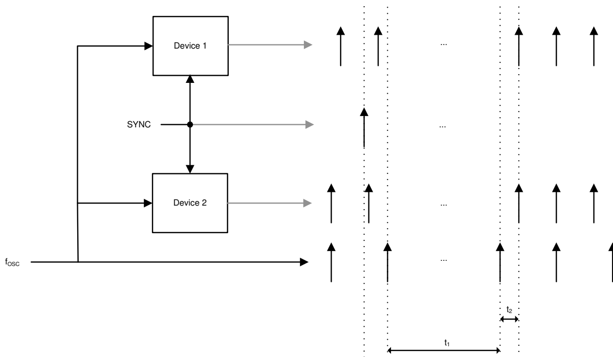
Figure 6-6. Devices Are Now Synchronized to OSCin Signal
