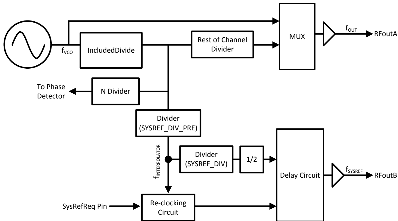
Figure 6-9. SYSREF Setup
