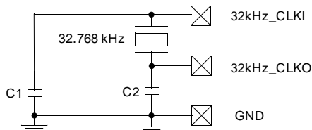
Figure 4. 32.768 kHz Oscillator
