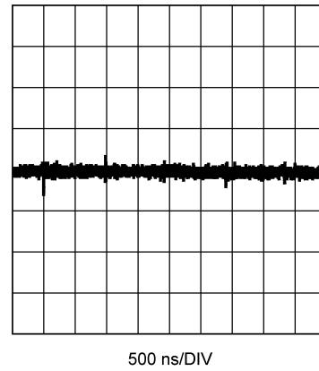
500 ns/DIV V_{IN} = 3.3\text{ V} , V_{OUT} = 2.5\text{ V} , I_{OUT} = 3\text{ A} , 20 mV/DIV Refer to Table 5 for BOM
