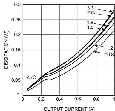
Figure 4. Dissipation 5-V Input at 25°C
