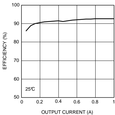
Figure 37. Efficiency
