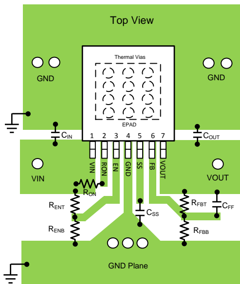
Figure 41. PCB Layout Guide
