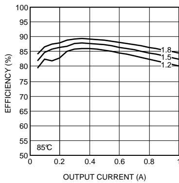
Figure 13. Efficiency 4.5-V Input at 85°C
