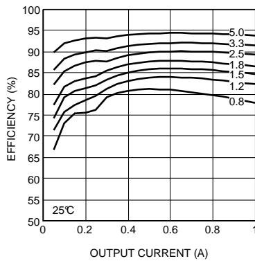
Figure 7. Efficiency 8-V Input at 25°C
