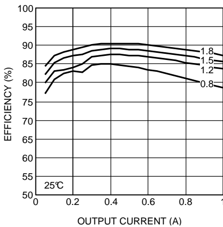
Figure 1. Efficiency 4.5-V Input at 25^\circ\text{C}
