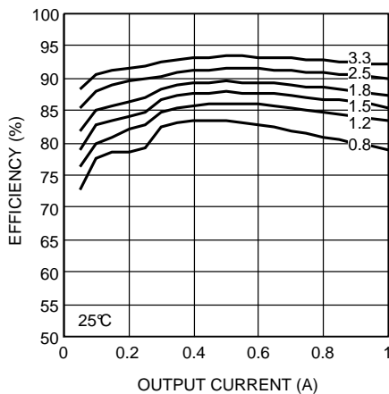
Figure 3. Efficiency 5-V Input at 25^\circ\text{C}
