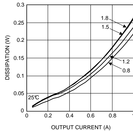
Figure 2. Dissipation 4.5-V Input at 25^\circ\text{C}
