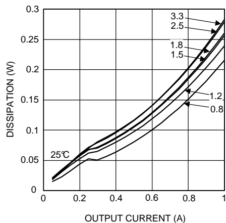
Figure 4. Dissipation 5-V Input at 25^\circ\text{C}
