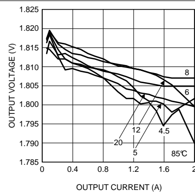
Figure 26. Line and Load Regulation at 85°C
