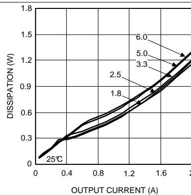
Figure 4. Dissipation 12-V Input at 25°C
