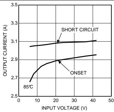
Figure 31. Current Limit 3.3- V_{OUT} at 85^\circ\text{C}
