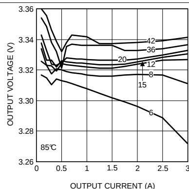
Figure 20. Line and Load Regulation at 85°C
