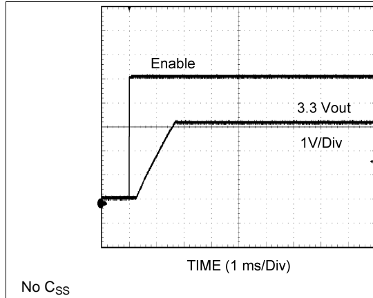
Figure 43. 3.3 V OUT Soft-Start
