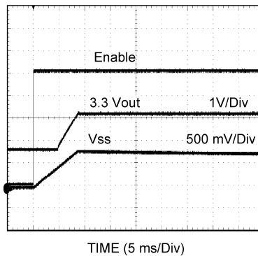
Figure 48. Prebiased Start-Up
