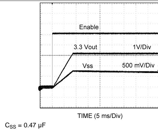
Figure 44. 3.3 V OUT Soft-Start
