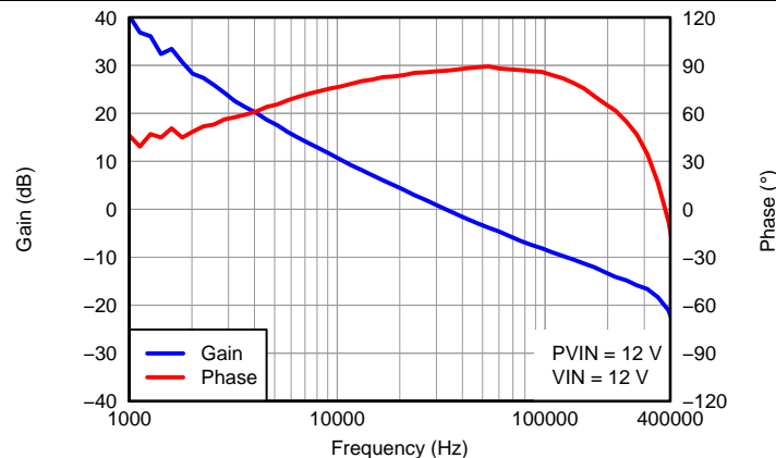
Figure 5. V OUT =1.2 V, I OUT =3 A, C OUT1 =47 µF ceramic, C OUT2 = 330 µF POSCAP, f SW =480 kHz
