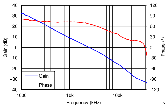
Figure 10. V OUT = 1.8 V, I OUT = 7 A, C OUT = 200 µF Ceramic, f sw = 500 kHz
