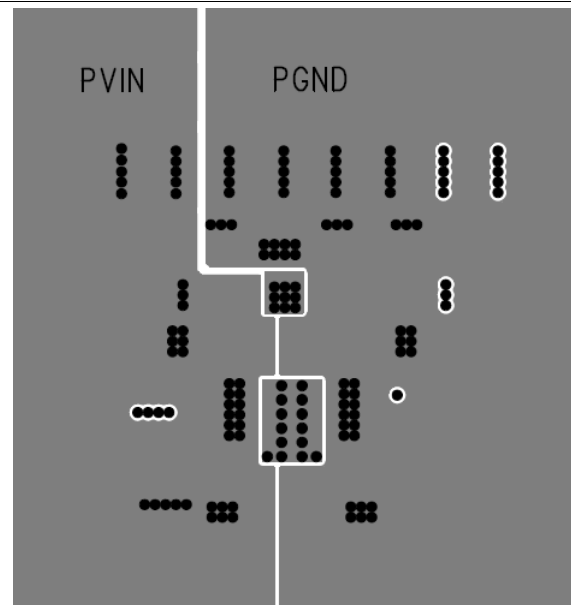
Figure 43. Typical Layer-2 Layout
