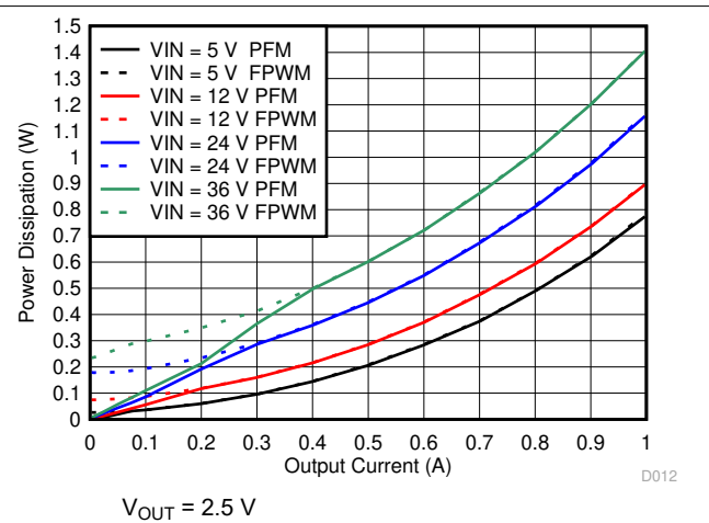
Figure 6-14. Power Dissipation
