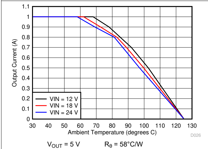
Figure 6-21. Ambient Temperature vs Output Current
