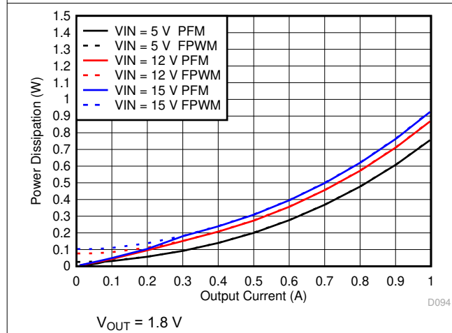
Figure 6-15. Power Dissipation
