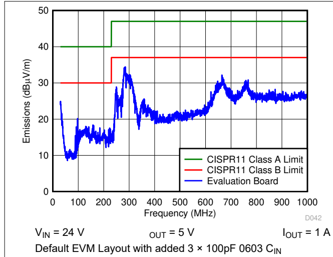
Figure 6-7. Radiated EMI
