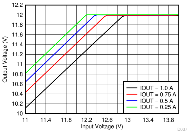
Figure 6-3. Dropout Voltage
