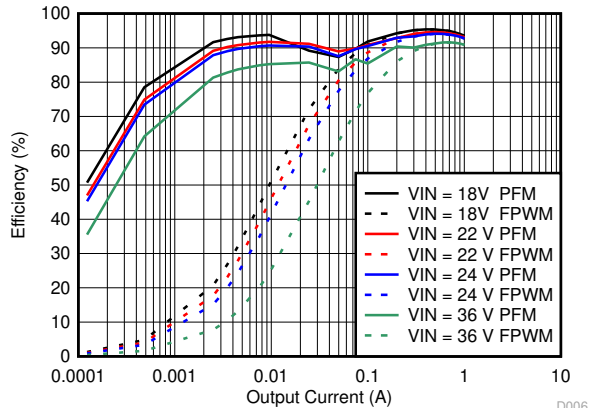
Figure 8-24. Efficiency
