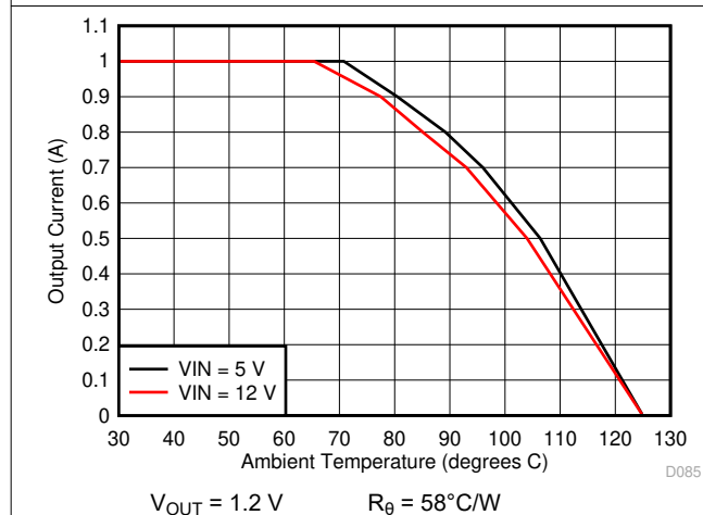
Figure 6-17. Ambient Temperature vs Output Current
