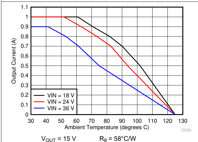
Figure 6-23. Ambient Temperature vs Output Current
