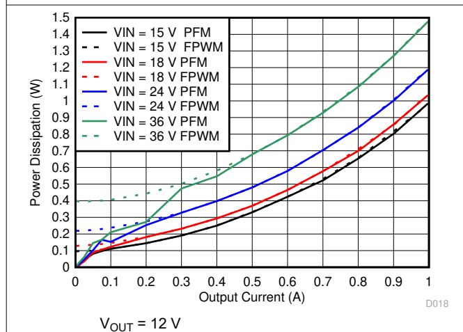
Figure 6-11. Power Dissipation
