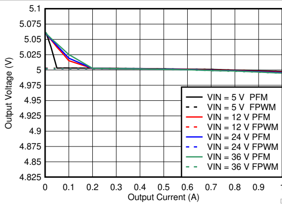
Figure 8-44. Line and Load Regulation for V_{OUT} = 5\text{ V}
