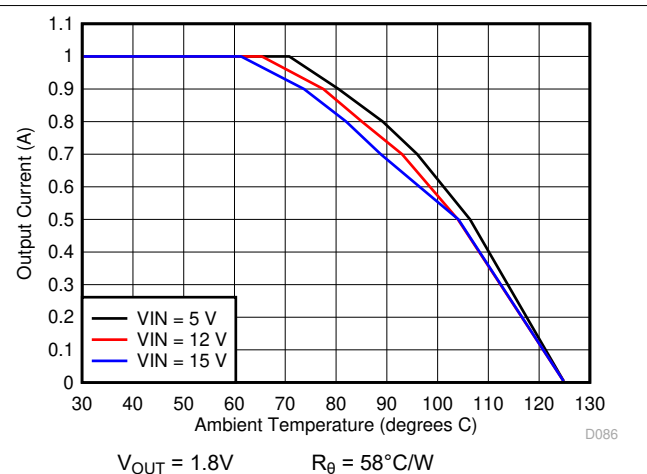
Figure 6-18. Ambient Temperature vs Output Current
