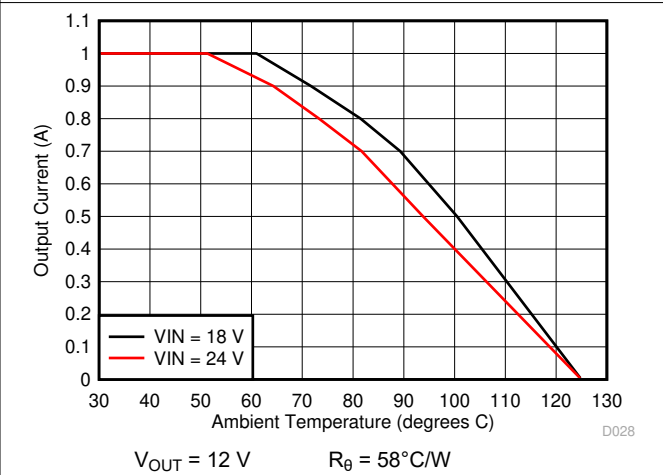
Figure 6-22. Ambient Temperature vs Output Current
