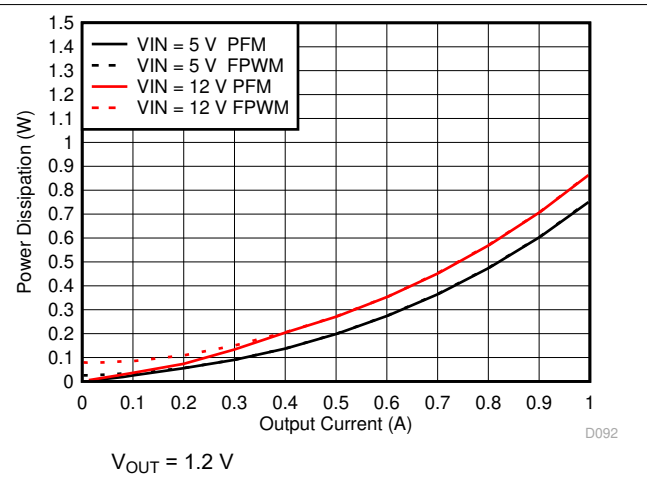
Figure 6-16. Power Dissipation
