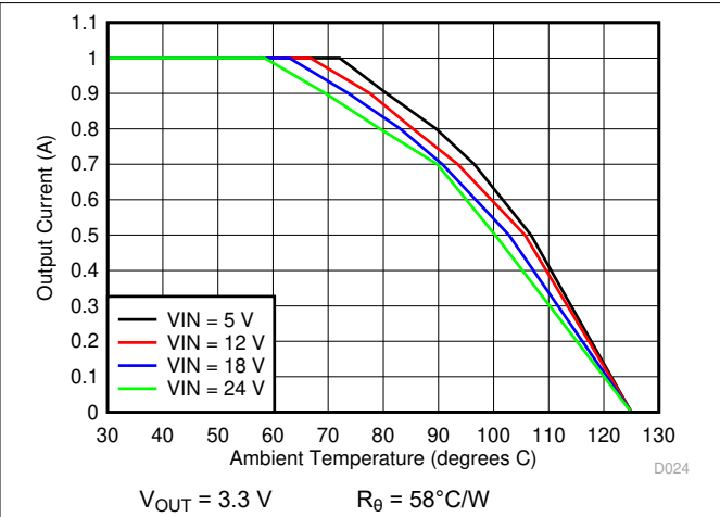
Figure 6-20. Ambient Temperature vs Output Current
