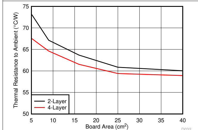
Figure 6-9. Package Thermal Resistance vs Board Copper Area, No Air Flow
