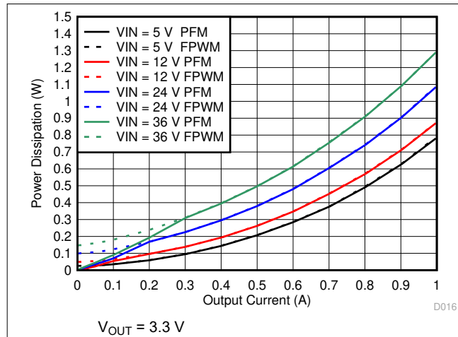
Figure 6-13. Power Dissipation
