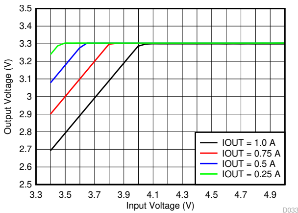
Figure 6-3. Dropout Voltage
