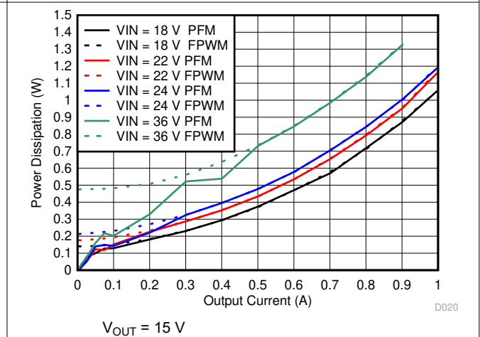
Figure 6-10. Power Dissipation
