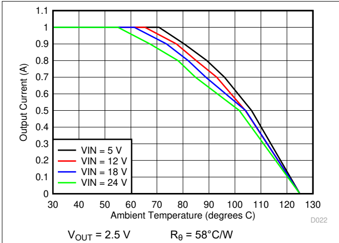
Figure 6-19. Ambient Temperature vs Output Current
