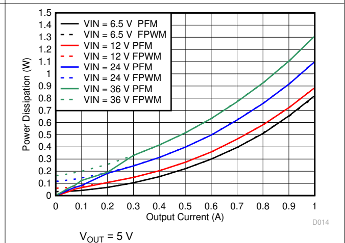
Figure 6-12. Power Dissipation
