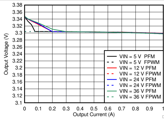
Figure 8-45. Line and Load Regulation for V_{OUT} = 3.3\text{ V}
