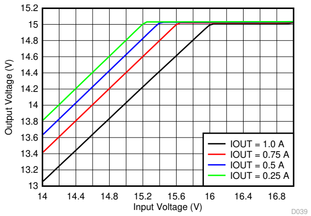
Figure 6-4. Dropout Voltage
