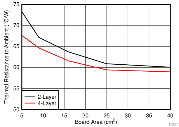
Figure 8-48. Package Thermal Resistance vs Board Copper Area
