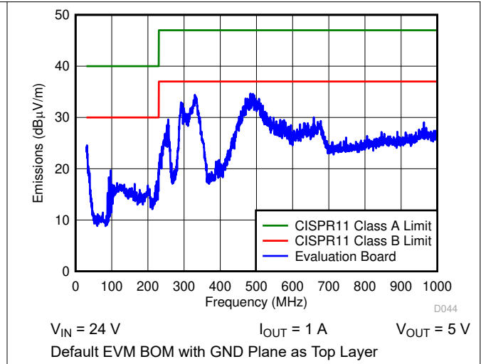
Figure 6-8. Radiated EMI
