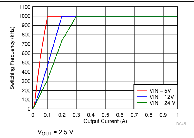
Figure 6-24. Auto PFM Mode Switching Frequency vs Output Current
