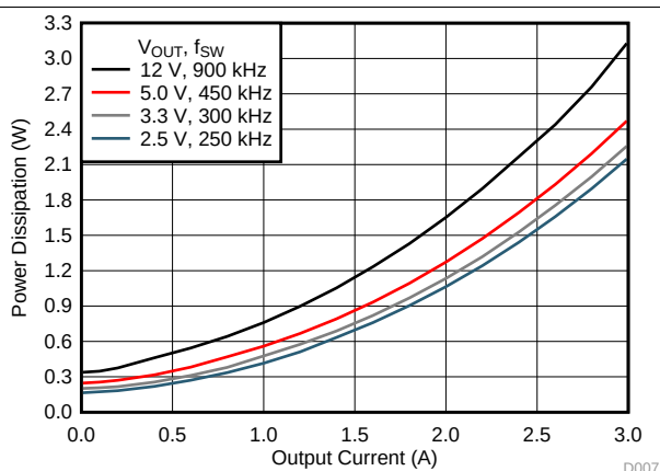
Figure 13. Power Dissipation vs Output Current
