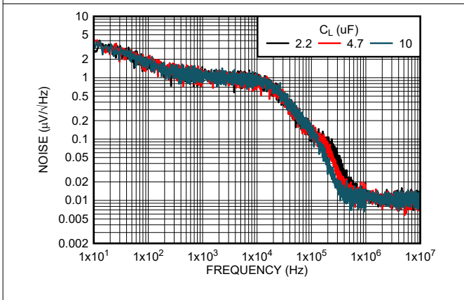
Figure 5-23. Output Noise Density vs Output Capacitor ( C_L ) and Frequency (New Chip)
