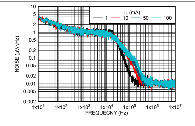
Figure 5-22. Output Noise Density vs Load Current ( I_L ) and Frequency (New Chip)
