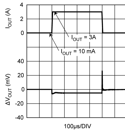
Figure 20. Load Transient
