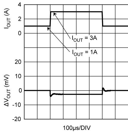
Figure 19. Load Transient
