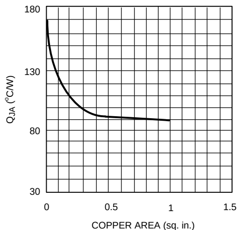
Figure 22. \theta_{JA} vs. Copper (1 ounce) Area for SOIC Package
