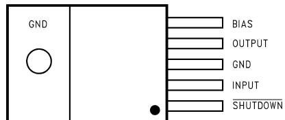
Figure 1. TO-220, Top View
