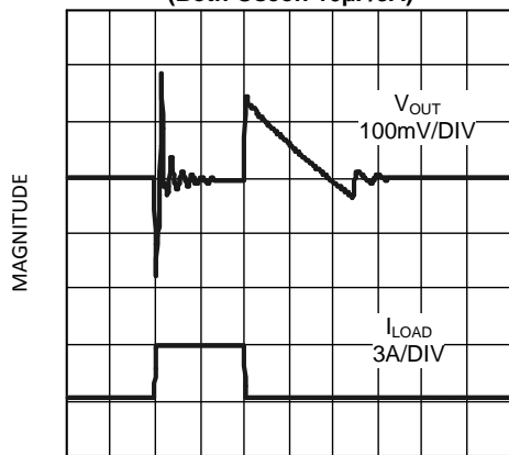
Load Transient Response (Both Oscon 10 \mu\text{F} /3A)
