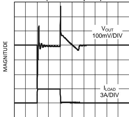
Load Transient Response (Tantalum 10 \mu\text{F} /3A)
