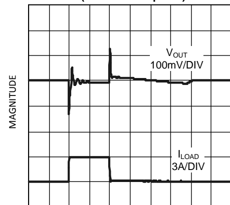
Load Transient Response (Tantalum 100 \mu\text{F} /3A)
