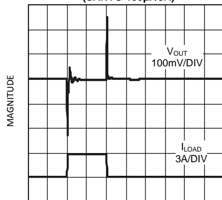
Load Transient Response (SANYO 150 \mu\text{F} /3A)
