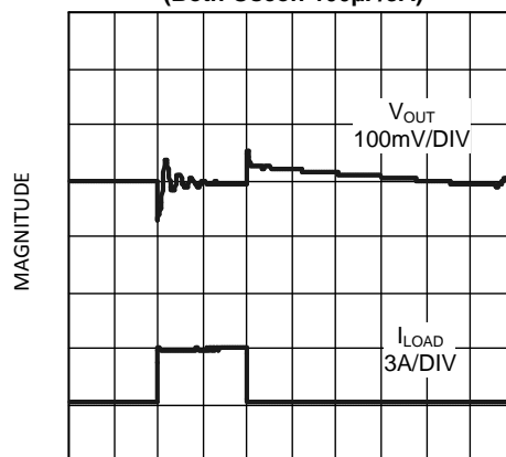
Load Transient Response (Both Oscon 100 \mu\text{F} /3A)
