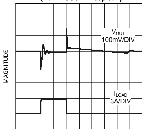
Load Transient Response (Both POSCAP 100 \mu\text{F} /3A)
