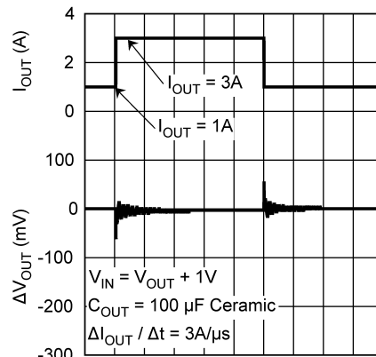
50 µs/DIV C OUT = 100-µF ceramic
