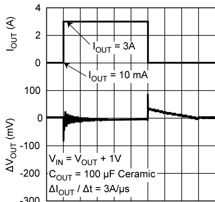
50 µs/DIV C OUT = 100-µF ceramic
