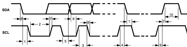
Figure 1. Timing Parameters
