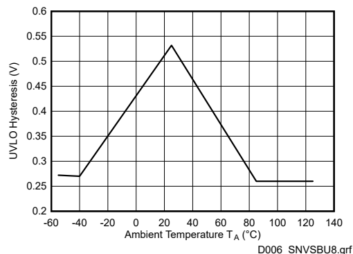
Figure 7-4. V_{CC} UVLO Hysteresis
