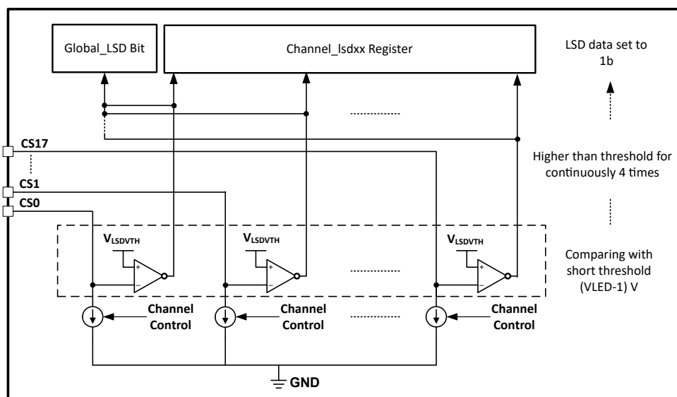
Figure 8-12. LSD Circuit
