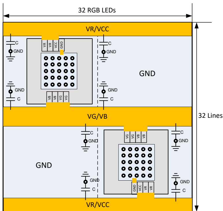
Figure 7-9. Power Rails Routing Suggestion
