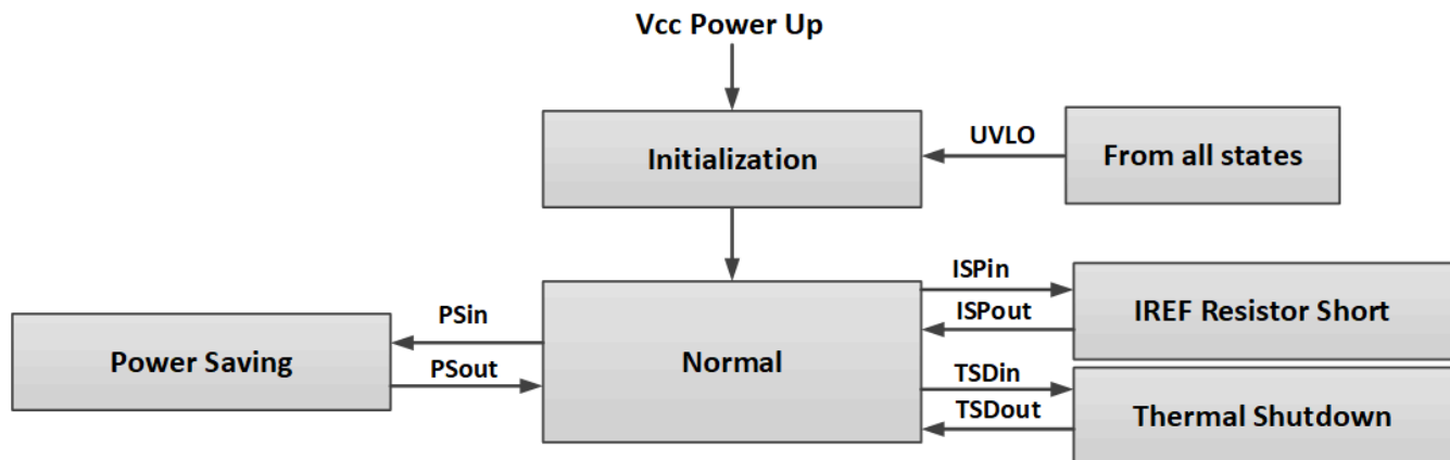
Figure 6-13. Functional Modes
