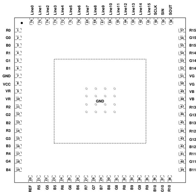
Figure 4-1. LP5892-Q1 RRF Package, 76-Pin VQFN With Exposed Thermal Pad (Top View)
