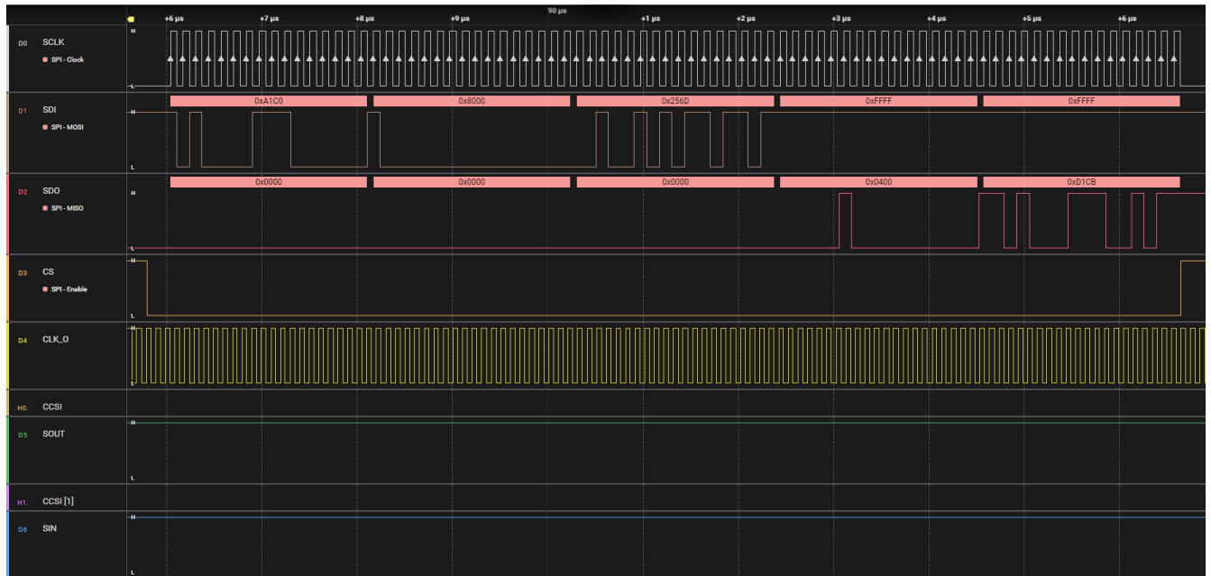
Figure 9-4. Write CLR_FLAG example
