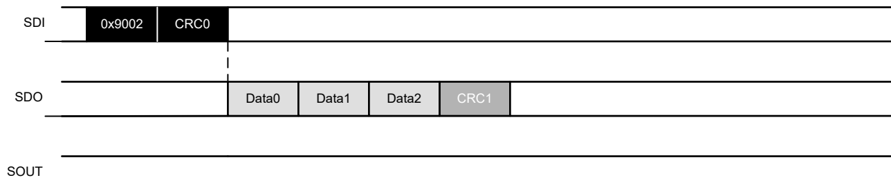
Figure 7-16. Example of DATA_RD command
