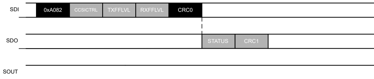
Figure 7-17. Example of REG_WR_CRC command
