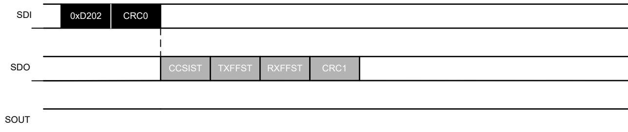
Figure 7-20. Example of REG_RD command
