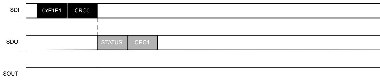
Figure 7-21. Example of SOFTRESET_CRC command
