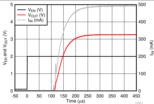
Figure 6-50. LP5912-3.3 Inrush Current
