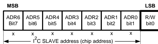
Figure 21. I²C Chip Address
