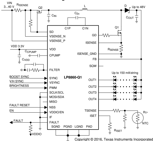
Simplified Schematic
