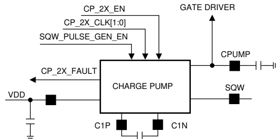
Figure 6-14. Charge Pump
