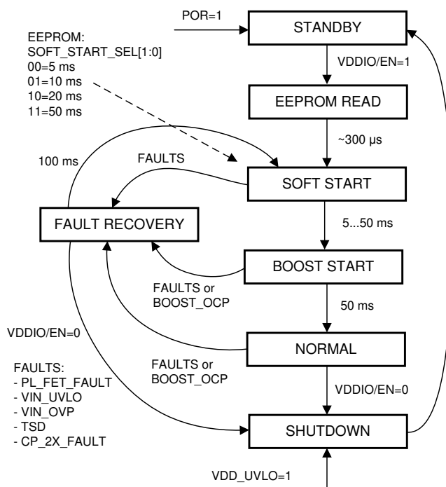
Figure 6-34. State Diagram
