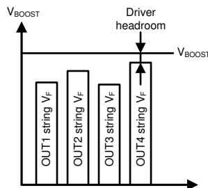
Figure 6-19. Boost Voltage Adaptation
