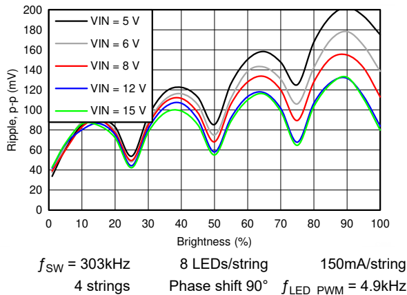
Figure 5-7. Boost Ripple
