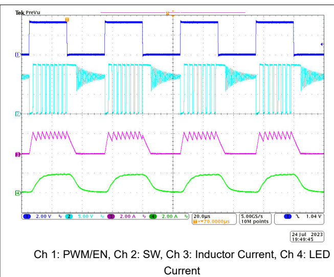
Figure 8-17. LED Current Ripple at PWM = 50%, 20kHz and F_{SW} = 400kHz
