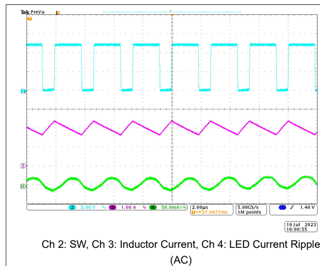
Figure 8-16. LED Current Ripple at ADIM = 100%, 1kHz and F_{SW} = 400kHz
